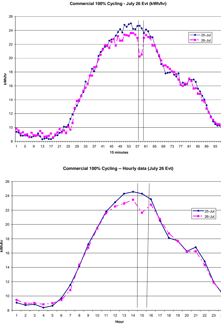
Figure 4-9: Small Commercial Hourly and 15-Minute Load Profiles (kWh/hr) – 100% Cycling; July 26 Event
