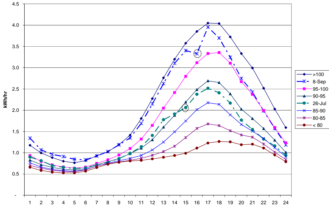
Residential SDP Loads by Temperature Day-Type and Event-Day (Valley C; 50% Cycling)
